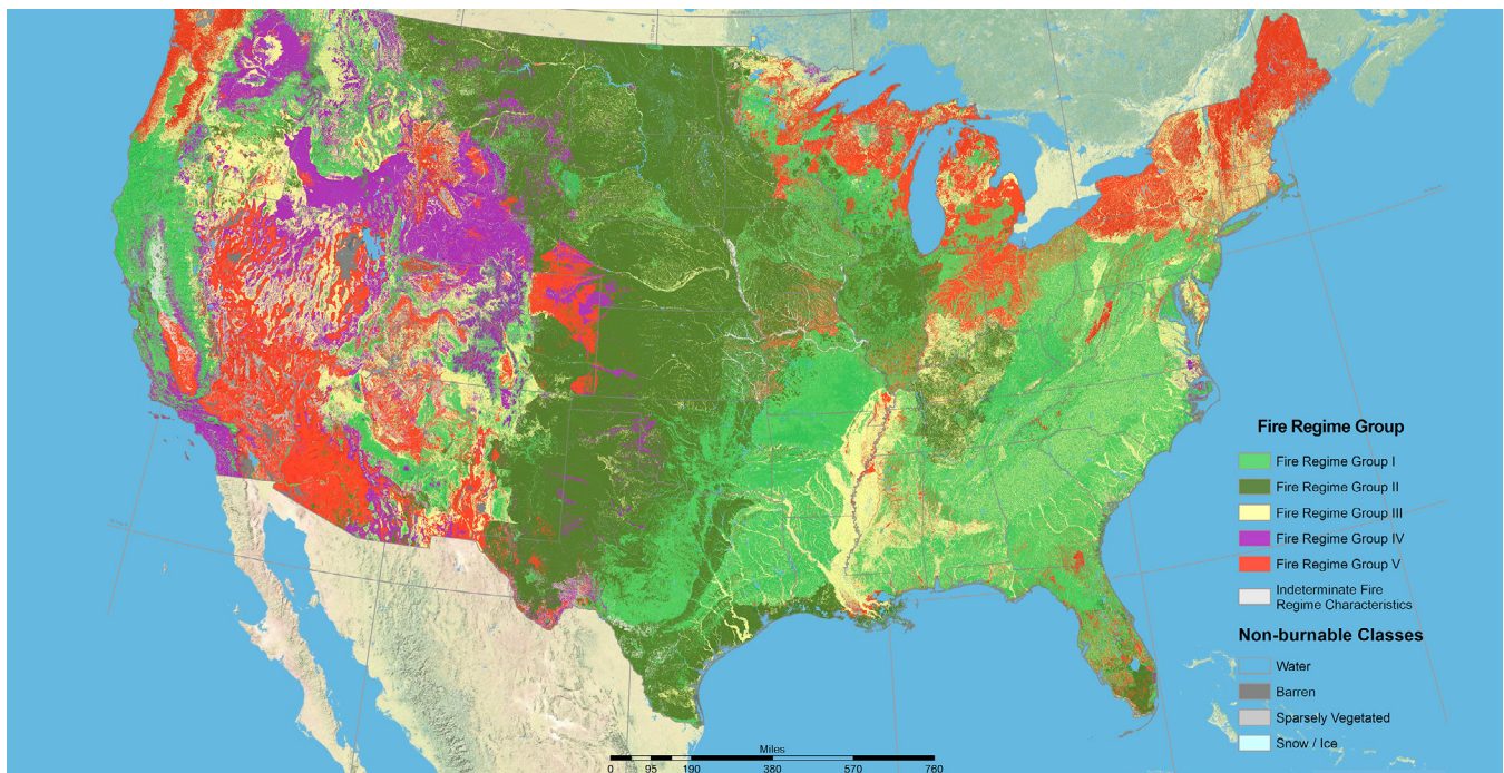
Figure 3. LANDFIRE Fire Regime Groups for the lower 48 US states. Data is publicly available at: https://www.landfire.gov/geoareasmaps/2012/CONUS_FRG_c12.jpg .
